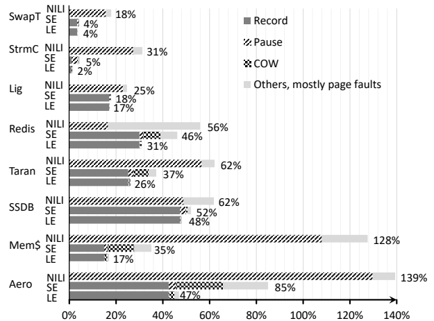
Figure 3: Performance overheads: NiLiCon, RRC-SE , RRC-LE .
