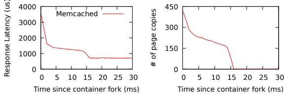
Figure 4: Average response latency and the number of COW since container fork.
